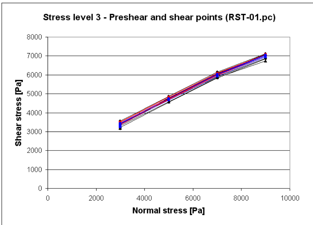
Fig. 5.7: Test points at stress level 3 (RST-01.pc, 16 yield locus tests)
