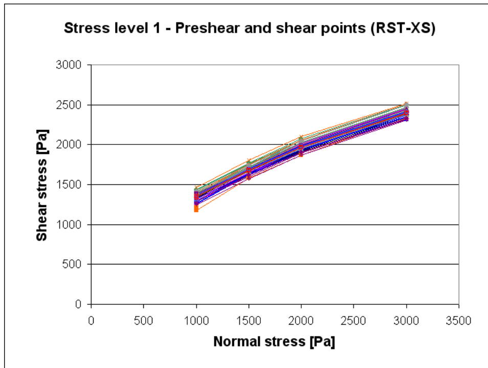
Fig. 5.1: Test points at stress level 1 (RST-XS, 60 yield locus tests)
