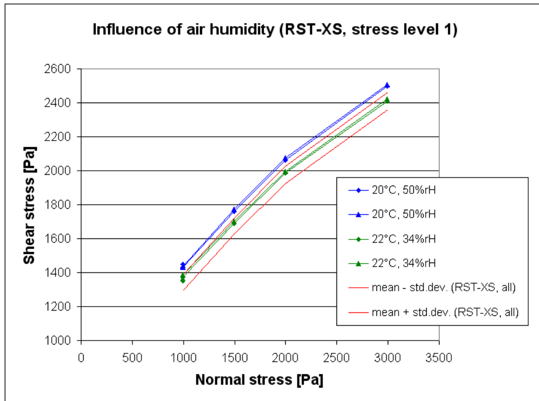
Fig. 5.14: Shear stresses measured at two different ambient conditions; range \tau_m \pm s (mean \pm standard deviation) of all RST-XS test results (red curves) for stress level 1
