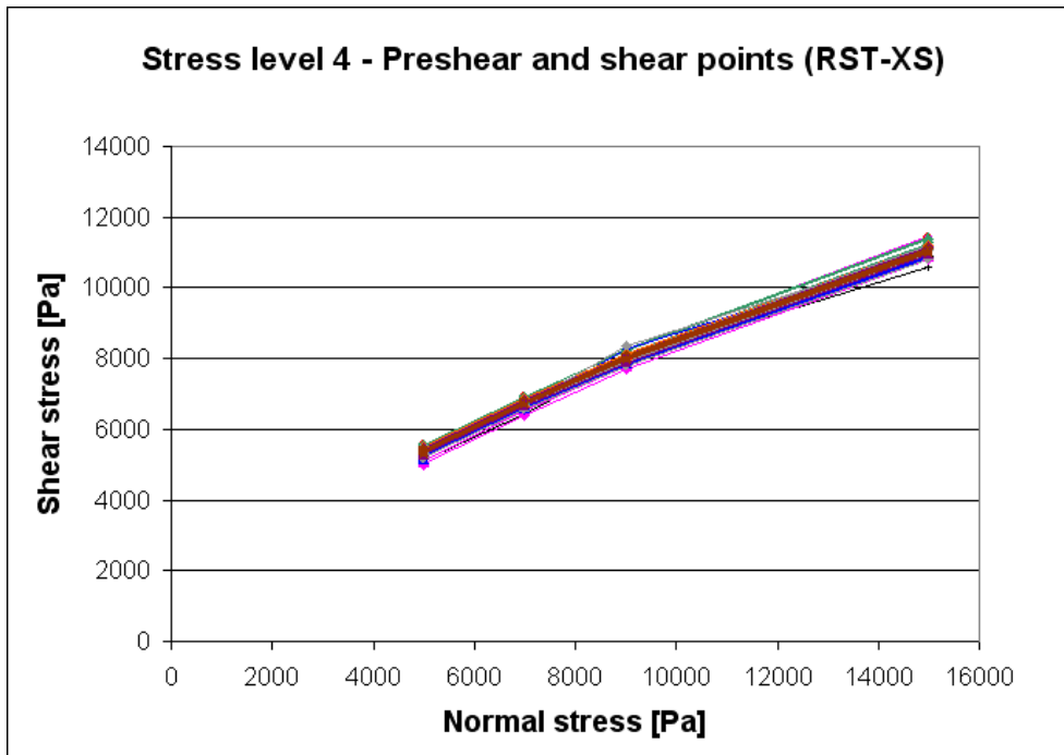
Fig. 5.4: Test points at stress level 4 (RST-XS, 52 yield locus tests)
