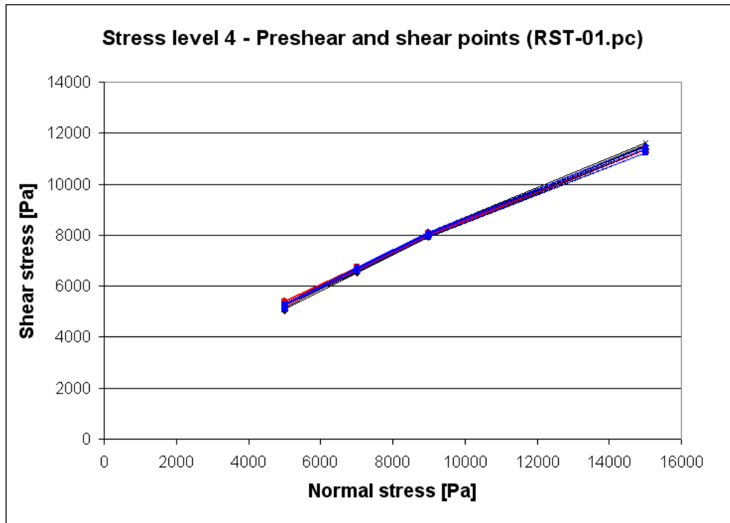
Fig. 5.8: Test points at stress level 4 (RST-01.pc, 16 yield locus tests)
