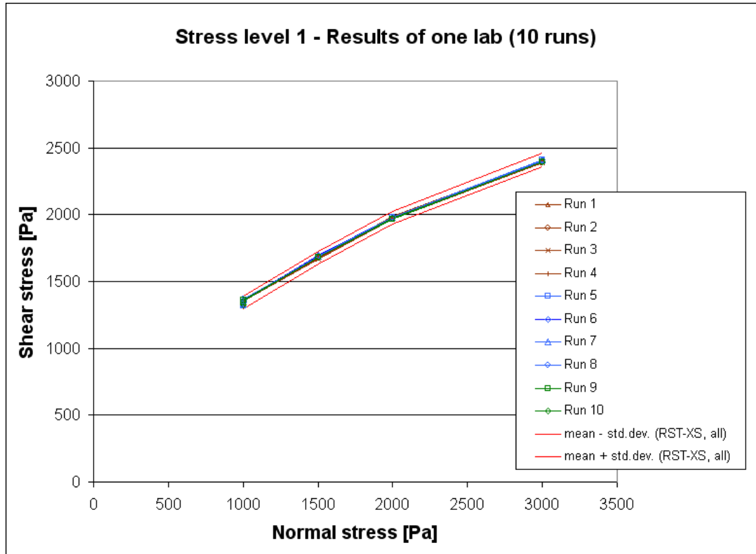
Fig. 5.15: Shear stresses measured by the lab having provided the largest number of test runs (storage of the limestone powder at 40%rH for run 1 to 5 and at 52%rH for run 6 to 10); range \tau_m \pm s (mean \pm standard deviation) of all RST-XS test results (red curves) for stress level 1
