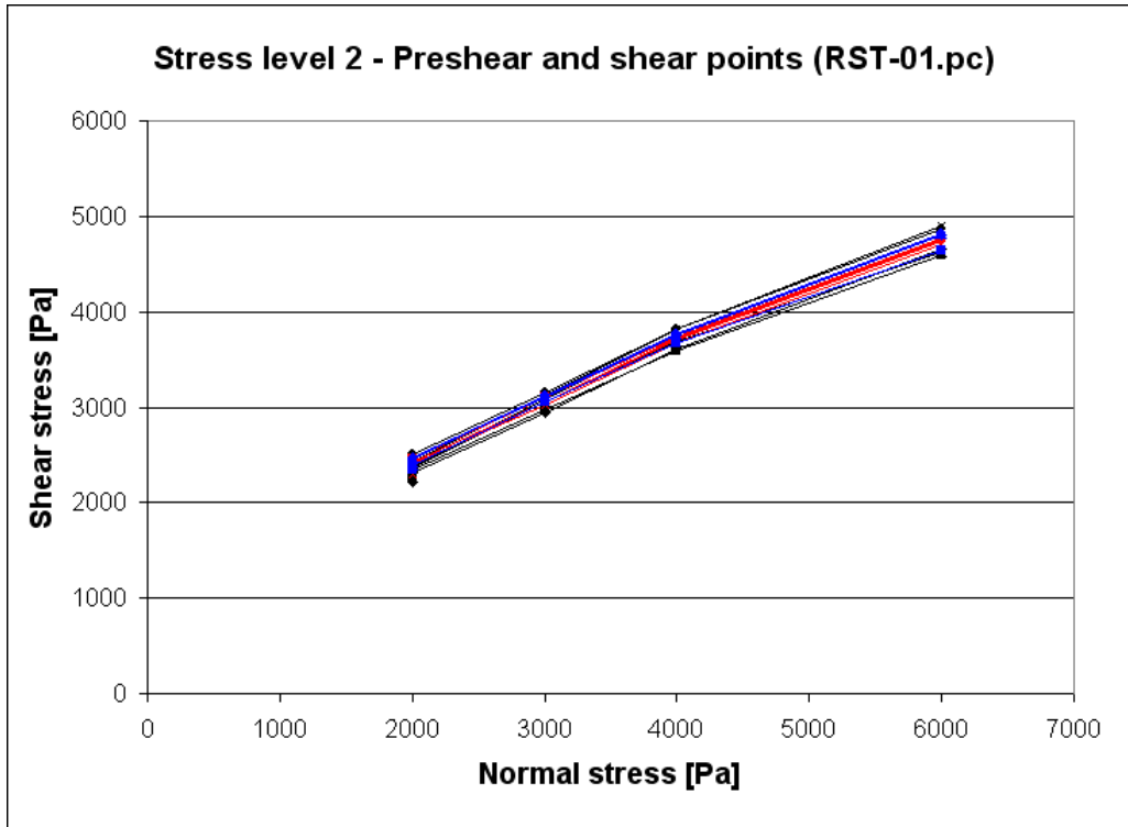
Fig. 5.6: Test points at stress level 2 (RST-01.pc, 17 yield locus tests)
