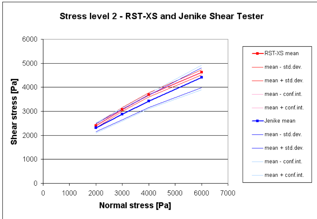
Abb. 5.9: Mean shear stress \tau_m (mean), range of standard deviation \tau_m \pm s (mean \pm std.dev.) and 95% confidence interval \tau_m \pm a (mean \pm conf.int.) of Jenike shear tester [2] (blue), ring shear tester RST-XS (red). Values have been measured at stress level 2.
