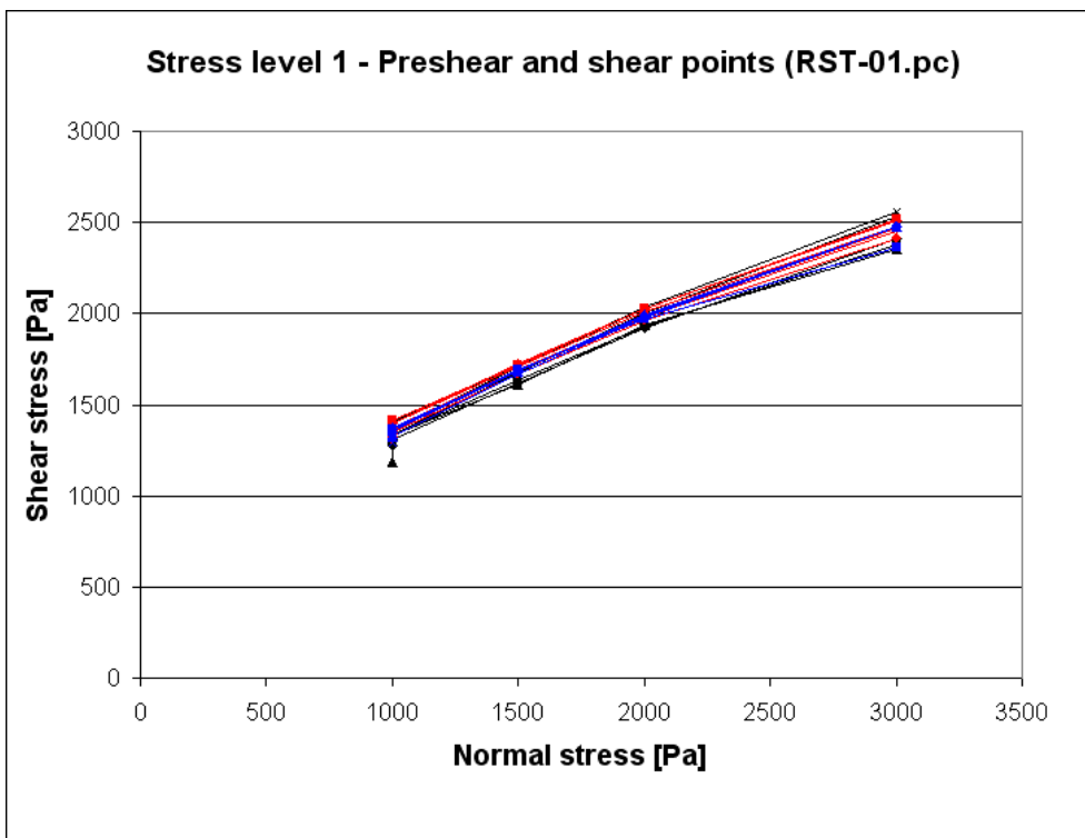
Fig. 5.5: Test points at stress level 1 (RST-01.pc, 19 yield locus tests)
