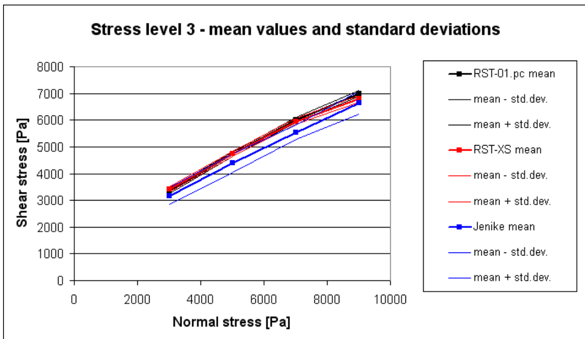
Fig. 5.12: Mean shear stress \tau_m (mean) and ranges \tau_m \pm s of standard deviation around mean (mean \pm std.dev.) of ring shear testers RST-01.pc (black) and RST-XS (red) and Jenike shear tester [2] (blue) for stress level 3
