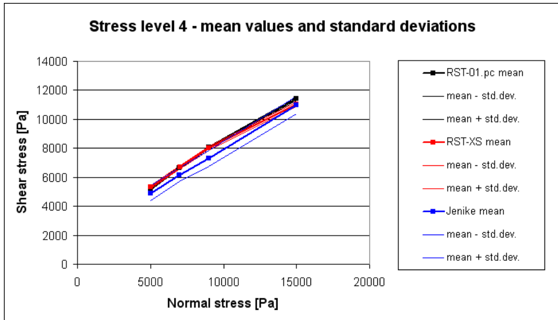
Fig. 5.13: Mean shear stress \tau_m (mean) and ranges \tau_m \pm s of standard deviation around mean (mean \pm std.dev.) of ring shear testers RST-01.pc (black) and RST-XS (red) and Jenike shear tester [2] (blue) for stress level 4
