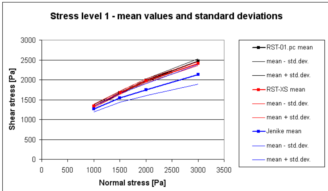
Fig. 5.10: Mean shear stress \tau_m (mean) and ranges \tau_m \pm s of standard deviation around mean (mean \pm std.dev.) of ring shear testers RST-01.pc (black) and RST-XS (red) and Jenike shear tester [2] (blue) for stress level 1
