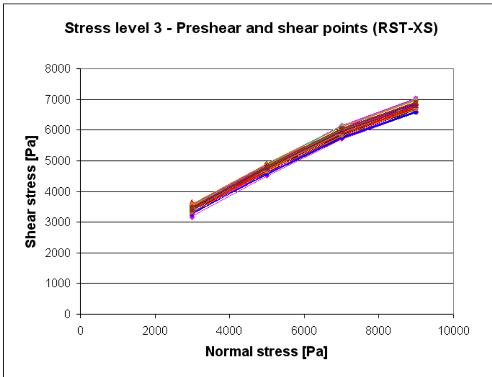
Fig. 5.3: Test points at stress level 3 (RST-XS, 52 yield locus tests)
