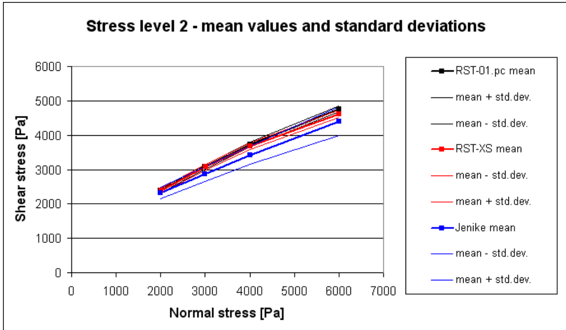
Fig. 5.11: Mean shear stress \tau_m (mean) and ranges \tau_m \pm s of standard deviation around mean (mean \pm std.dev.) of ring shear testers RST-01.pc (black) and RST-XS (red) and Jenike shear tester [2] (blue) for stress level 2
